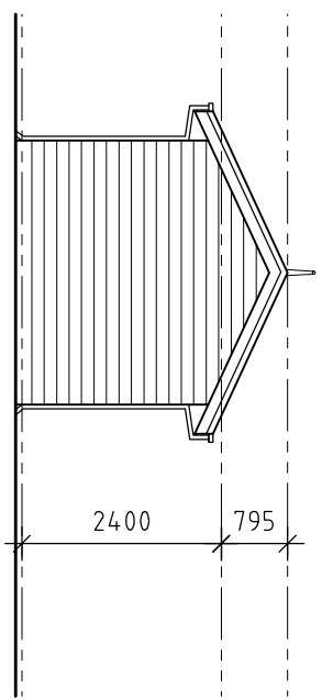
E REAR ELEVATION 1:50
