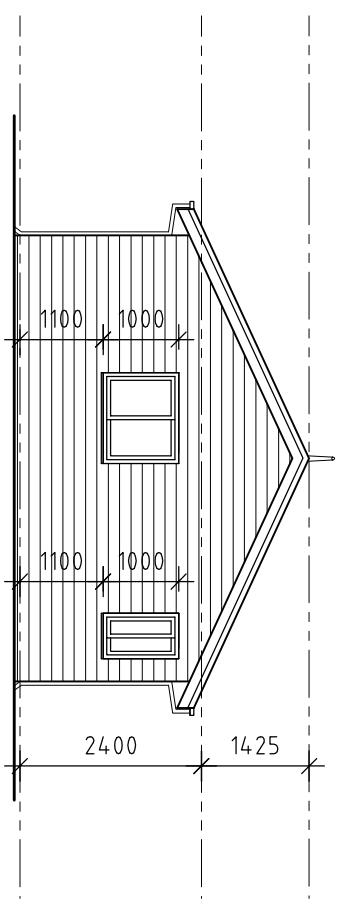
E REAR ELEVATION 1:50
