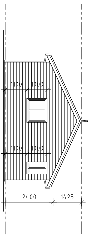
E REAR ELEVATION 1:50
