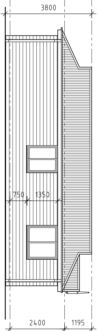
B SIDE ELEVATION 1:50
