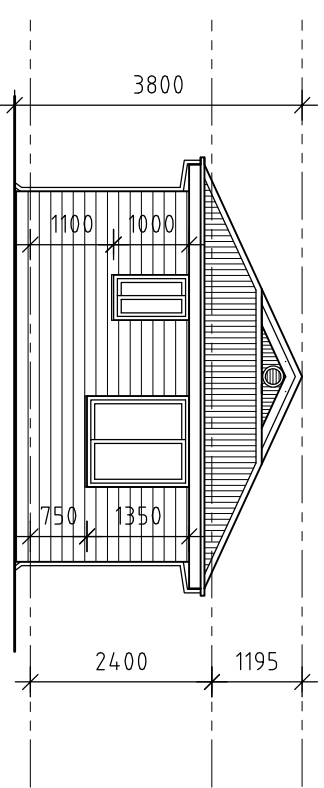
E REAR ELEVATION 1:50
